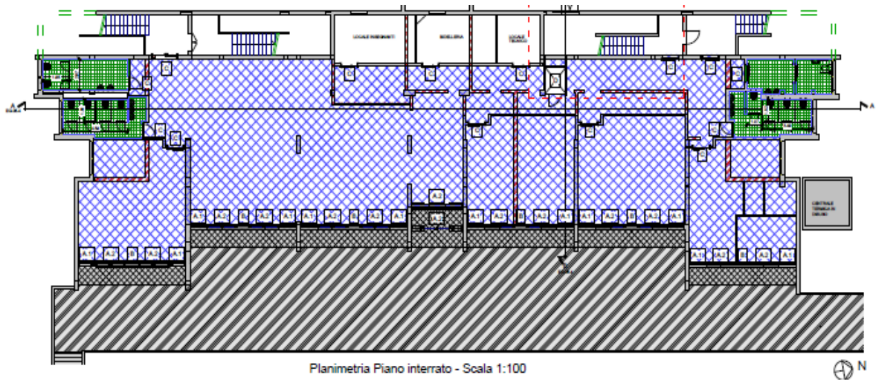
Iqbal Masih - Planimetria Piano Interrato
